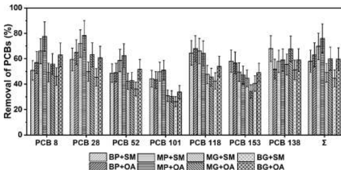
Fig. 5 Removal of PCBs by Fe-BNPs derived from Blaifränkisch grape berries (BG), and pomace (BP), Merlot grape berries (MG), and pomace (MP), and subsequently added bacterial strains O. anthropi (OA) or S. maltophilia (SM)
