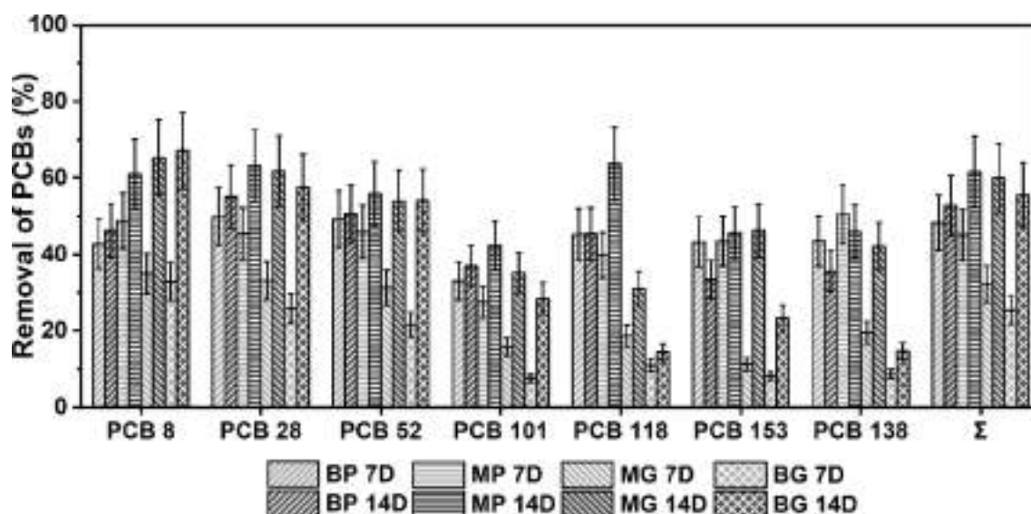
Fig. 4 Removal of PCBs by Fe-BNPs derived from Blaifränkisch grape berries (BG), Blaifränkisch grape pomace (BP), Merlot grape berries (MG) and Merlot grape pomace (MP)
